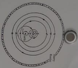
Figure 3: The Geocentric Model
